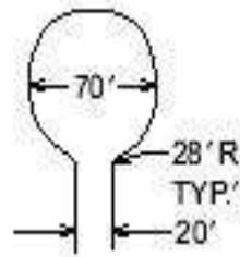
70' DIAMETER CUL-DE-SAC
